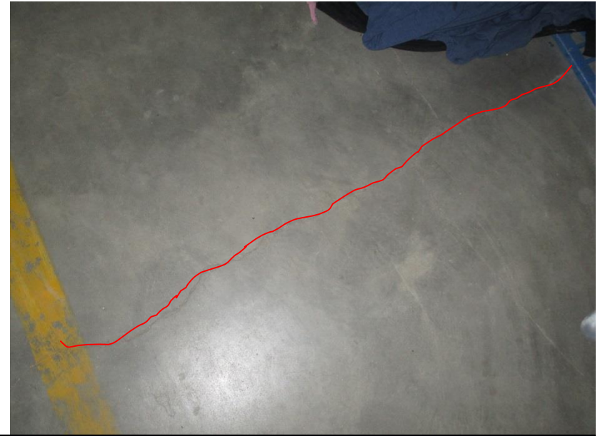
Hairline crack on slab
