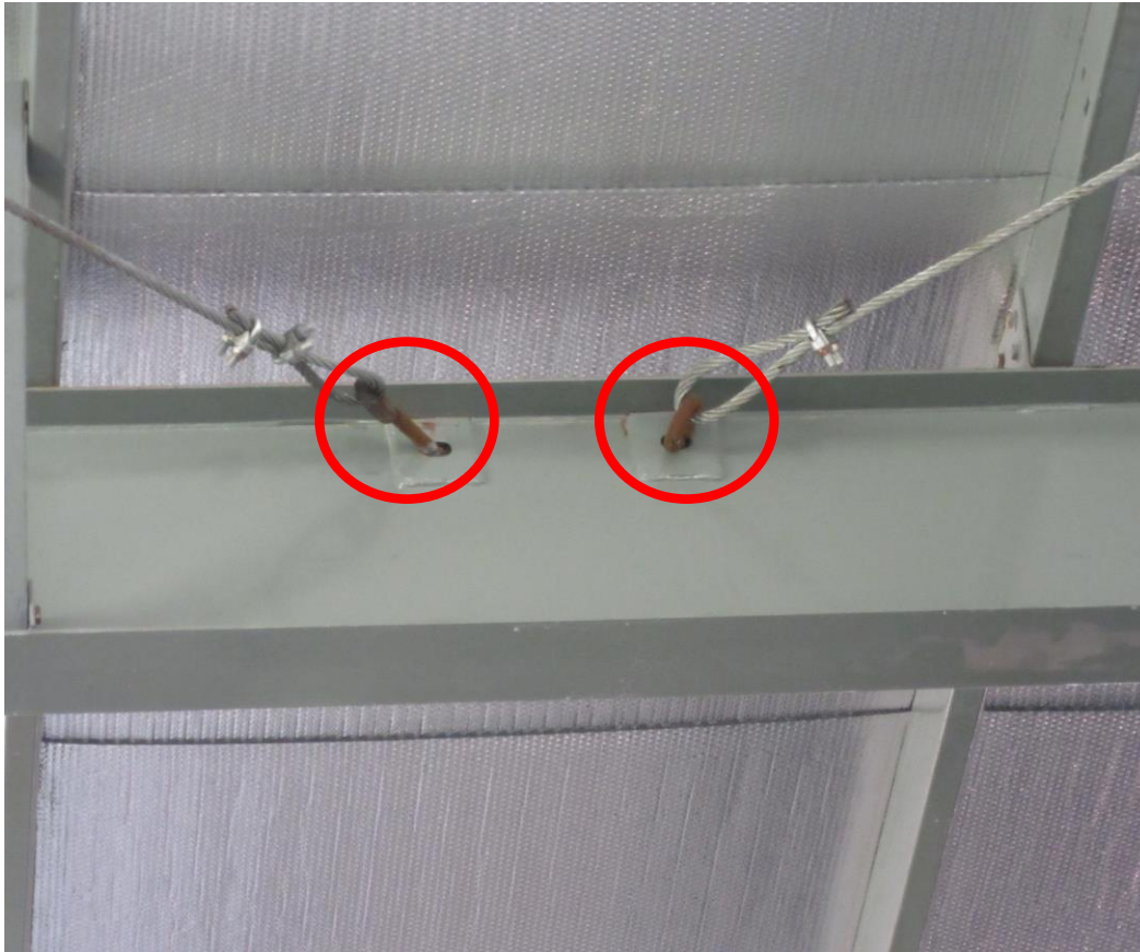
Corroded Parts of Bracing Cables
