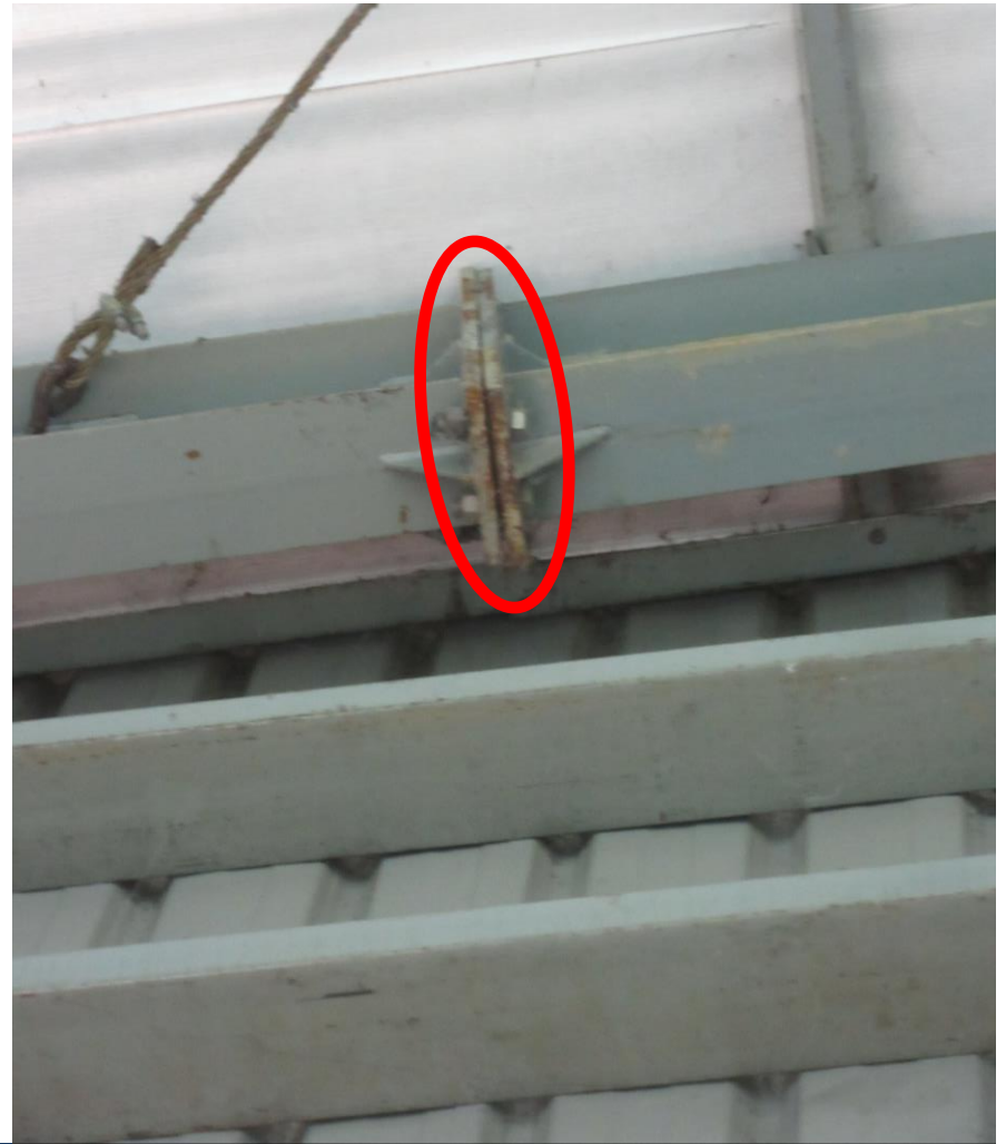
Gaps between End Plates of Frame Beam Splice Connections
