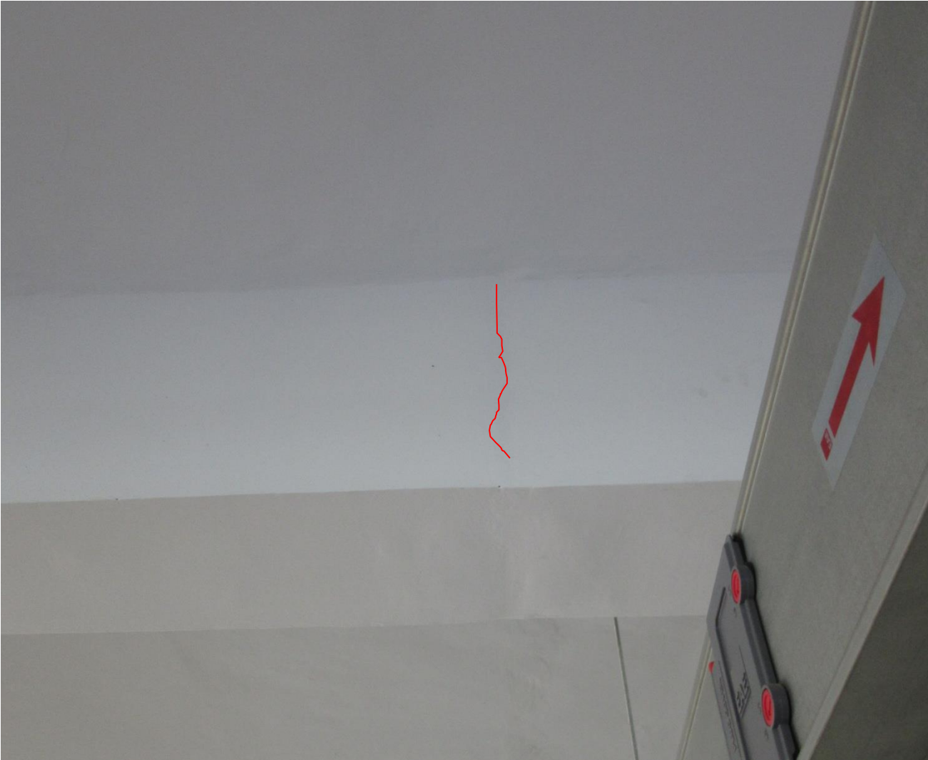
Hairline crack observed on a beam at 5 th floor ceiling.
