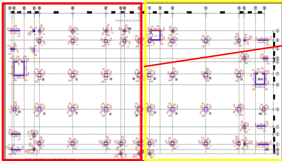
Provided Column layout plan
