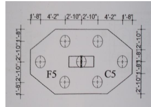
Foundation detail
