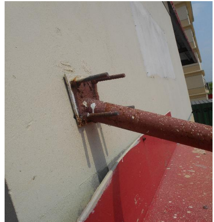
Connection between tension member and the brick façade wall.
