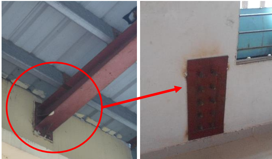
Rafter connected with brick façade.
