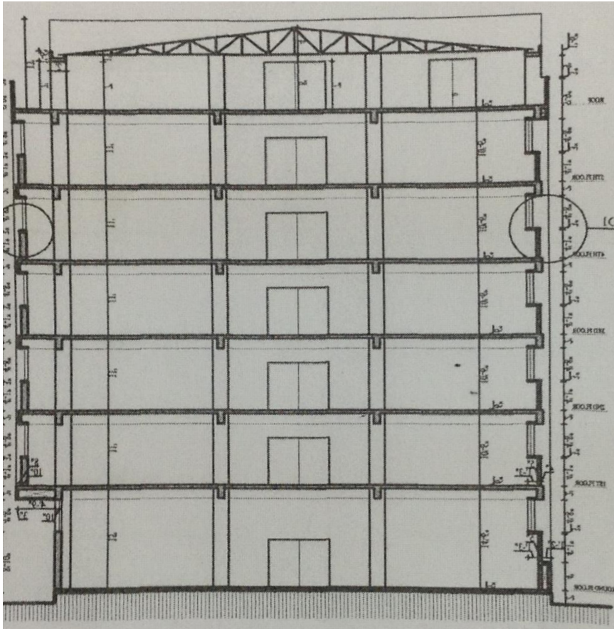
Steel roof structure replaced with concrete
