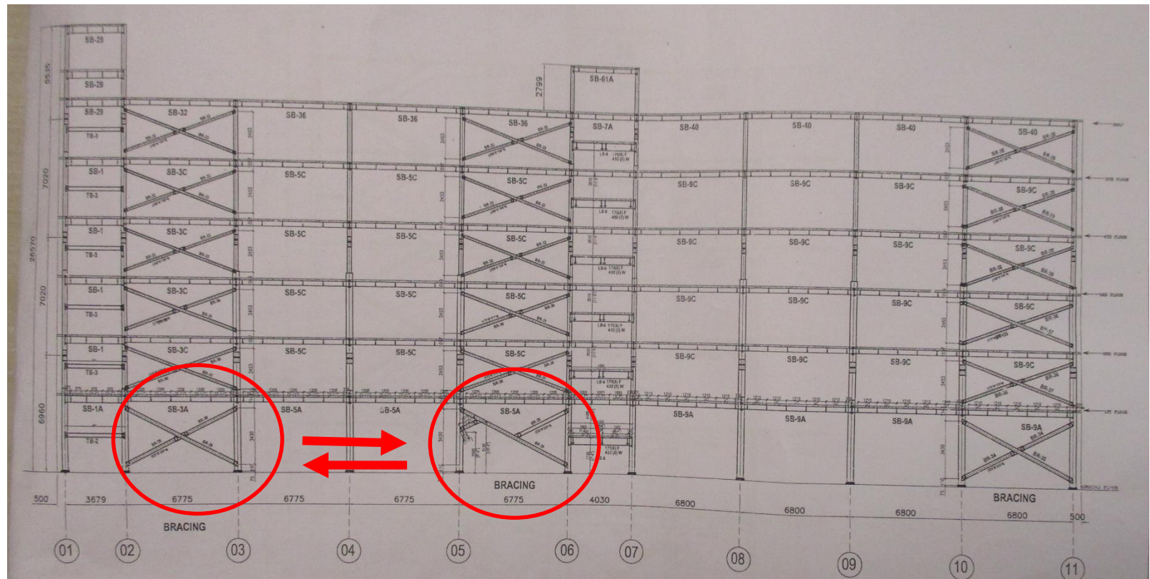
Cross section of Grid-A
