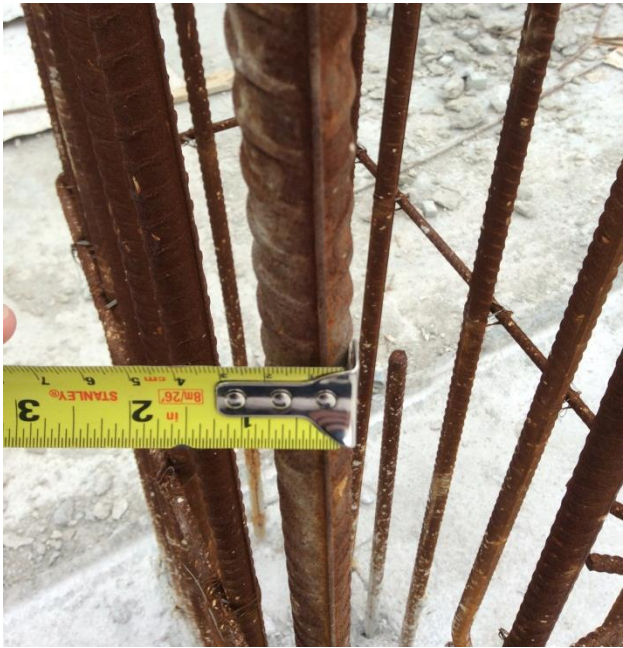
High strength rebar was observed in the column reinforcement at 4 rd floor
