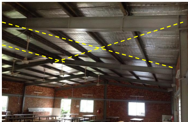
Dining room shed roof structure
